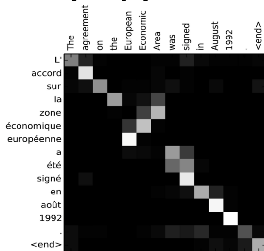
Figure 1: Attention mechanism showing mapping of French and English sentences
